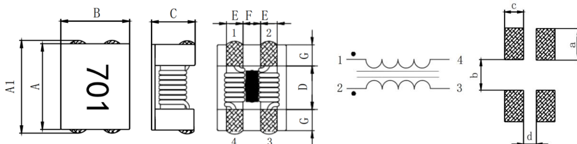
Electrical Schematic and PAD Layout
